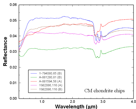
Fig. 2. Bidirectional VNIR reflectance spectra of the spots shown in Fig. 1, wherein three to five absorption bands are detected near 2.8 \mu\text{m} .
