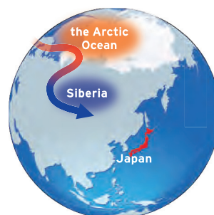
Meandering westerlies are involved in the "Warm Arctic, Cold Continents" trend pattern.
