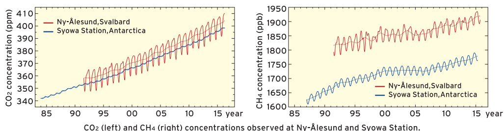
CO 2 (left) and CH 4 (right) concentrations observed at Ny-Ålesund and Syowa Station.
