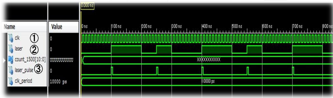
Fig.2.Result of Counter simulation
