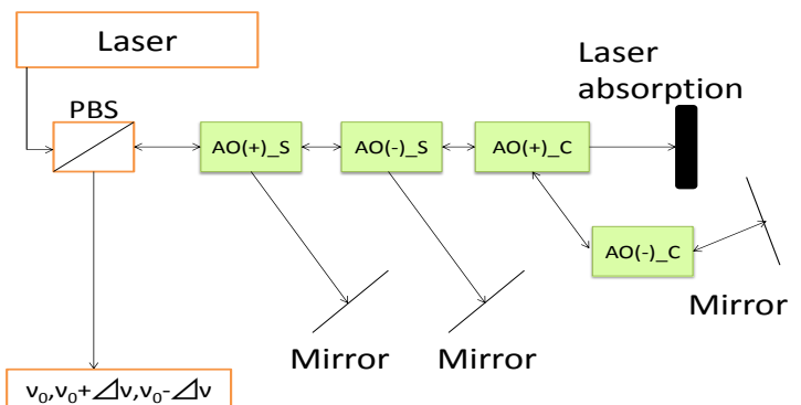
Fig.1. Schematics of the AO frequency shifter
